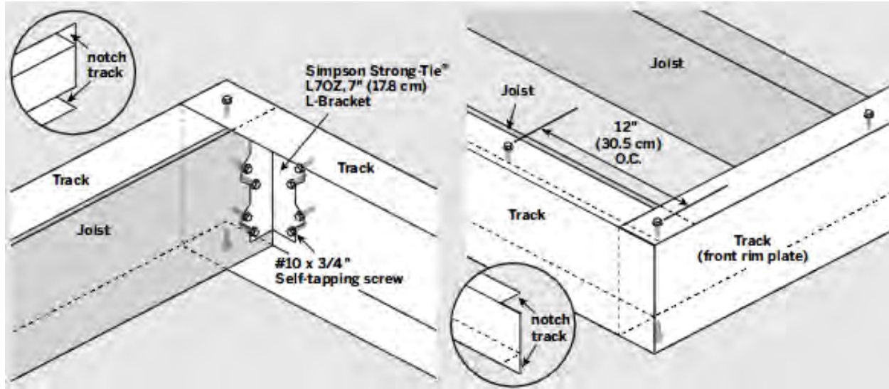
FIGURE 9 – 1-5/8 JOIST TO TRACK/LEDGER AND JOIST TO TRACK (FRONT PLATE) CONNECTION DETAILS
