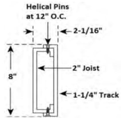
SINGLE BOX BEAM
