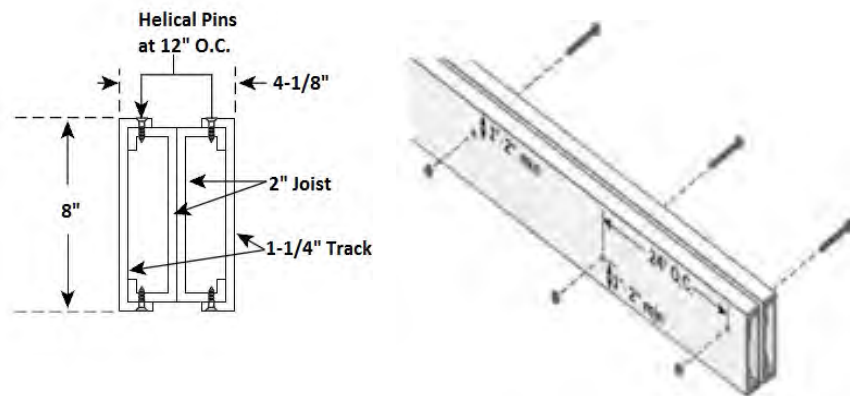
DOUBLE BOX BEAM
