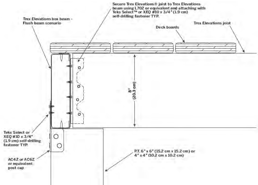
FIGURE 7 – 1-5/8 JOIST TO BOX BEAM CONSTRUCTION DETAIL – FLUSH BEAM SCENARIO
