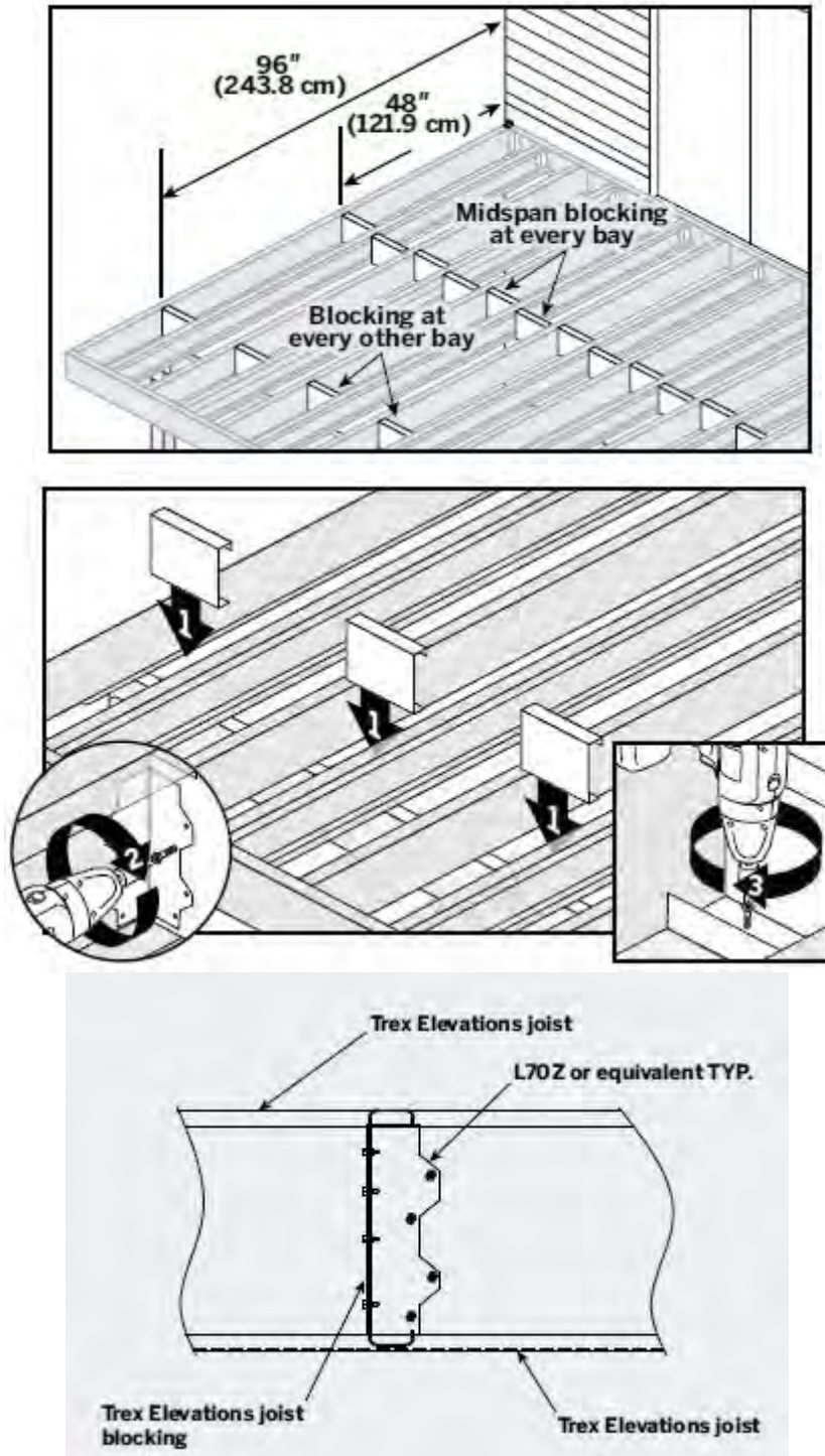
FIGURE 6 – 1-5/8 JOIST BLOCKING DETAILS
