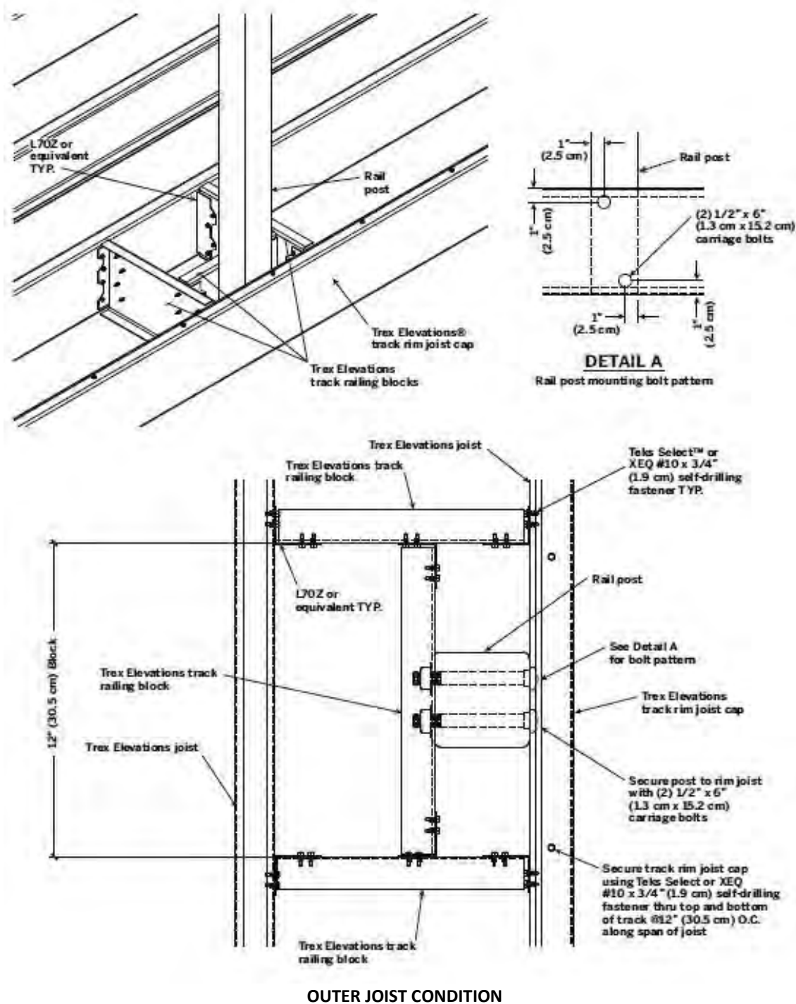
FIGURE 11 – RAIL POST INSTALLATION DETAILS
