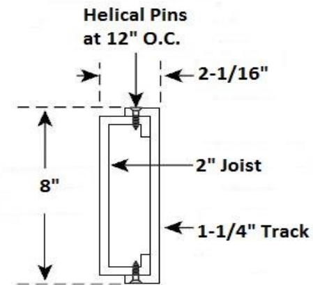
Figure 4 – Track/Ledger
