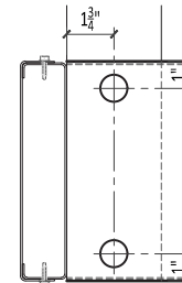
Bolt Pattern B
