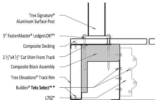
Surface Mount Assembly
