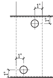
Bolt Pattern A
