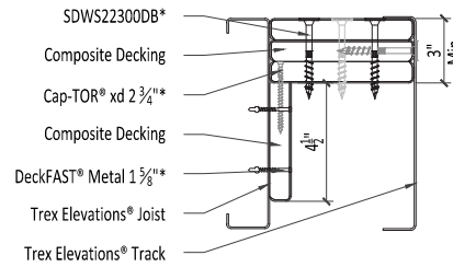
Composite Block Assembly
