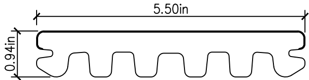
2 1 ENHANCE 1x6 GROOVED EDGE BOARDS NOT-TO-SCALE
