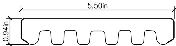
1 1 ENHANCE 1x6 SQUARE EDGE BOARDS NOT-TO-SCALE
