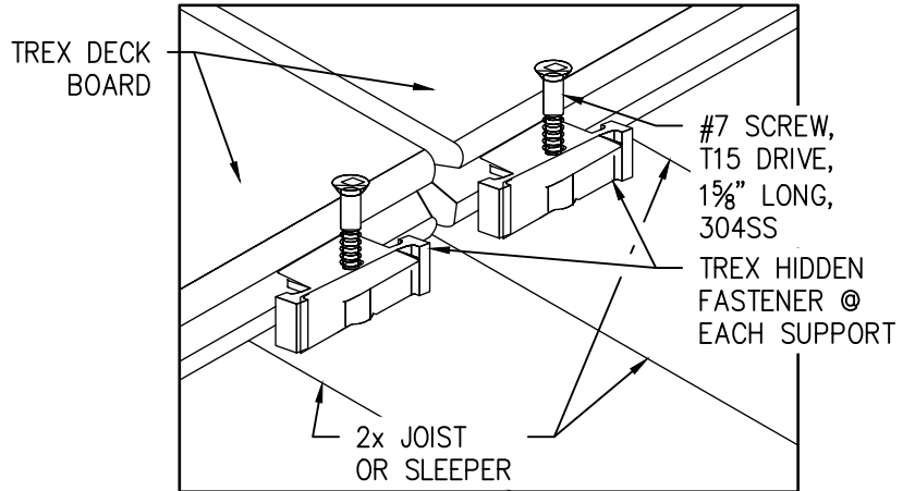
3 1 TYP. TREX HIDDEN FASTENER INSTALLATION NOT-TO-SCALE
