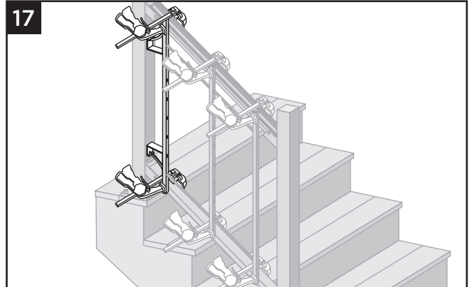
17. Clamp top vertical (upper part of stairs) in place, using width of stair template to position.
